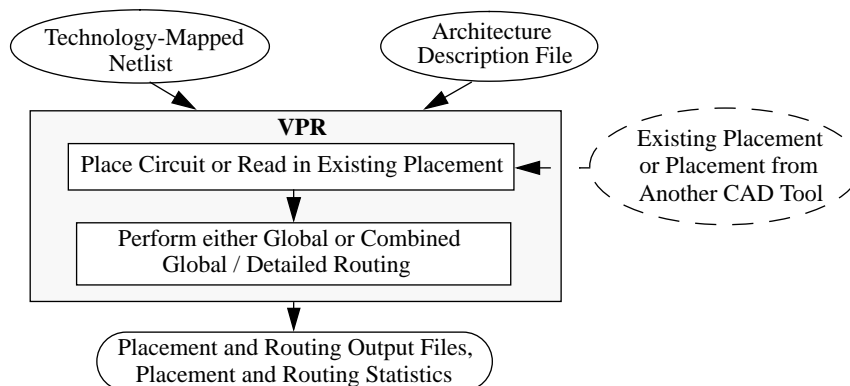
Fig. 1. CAD flow.
